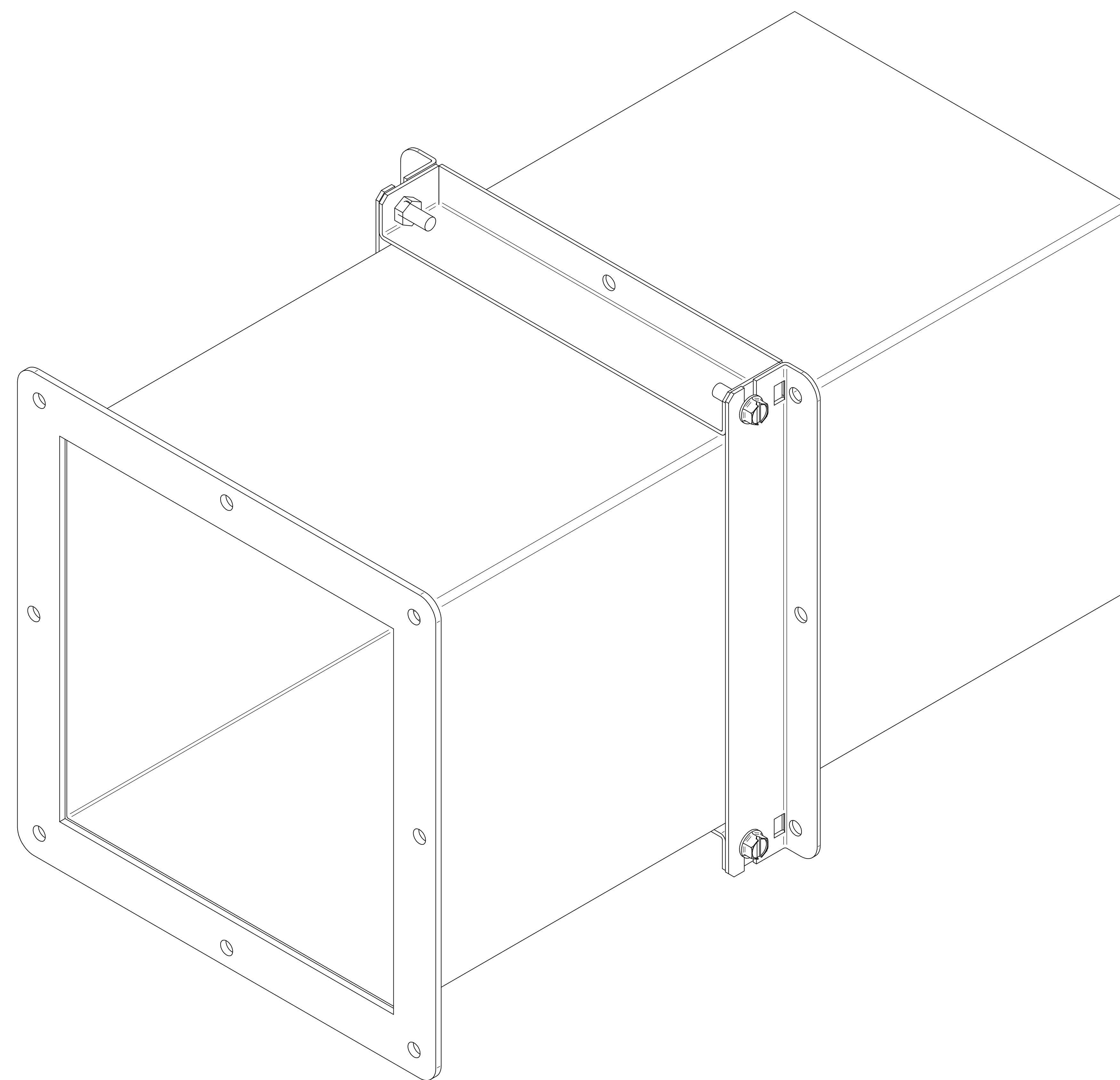
ISOMETRIC VIEW
