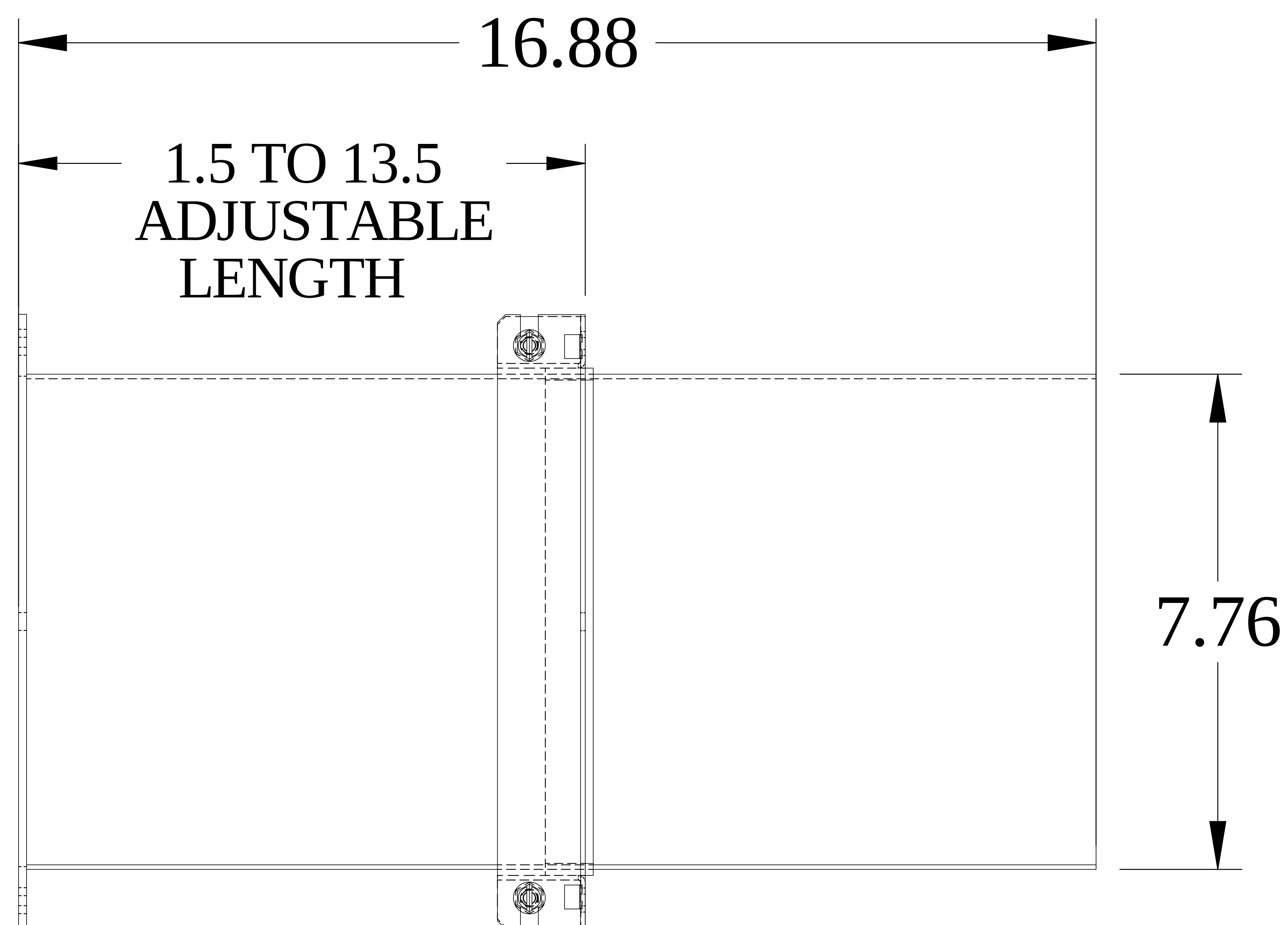
SIDE VIEW
