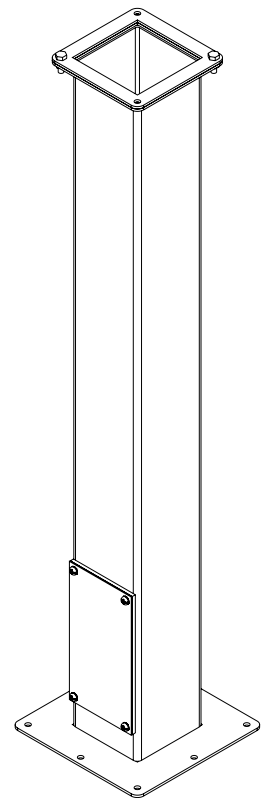
ISOMETRIC VIEW
