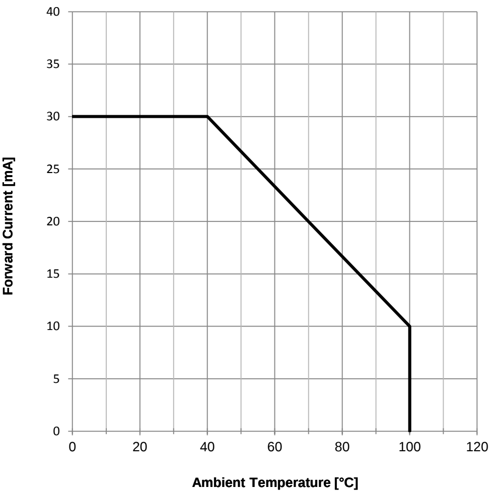
Derating Curve:
