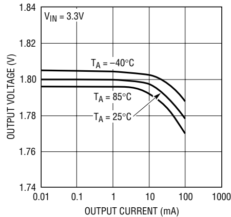
LTC1503-1.8 Output Voltage vs Output Current
