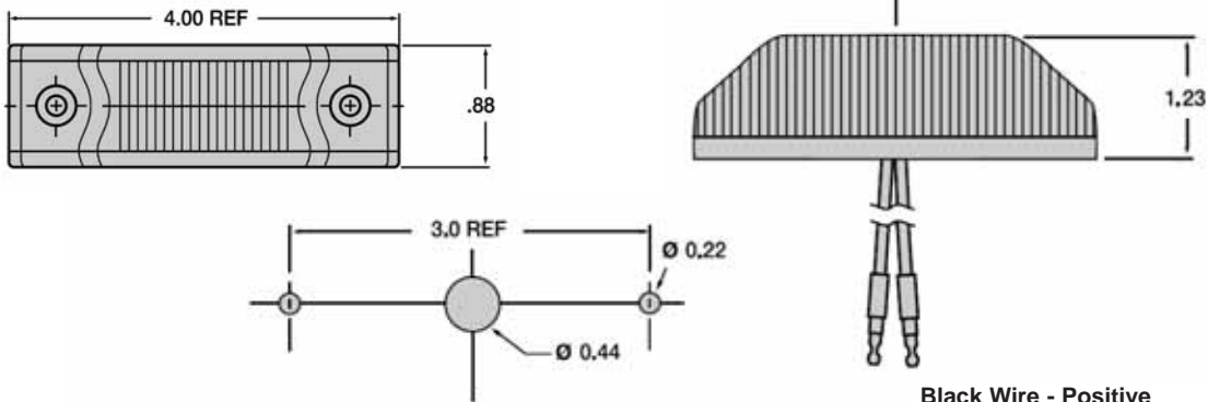
RECOMMENDED MOUNTING HOLE PATTERN
