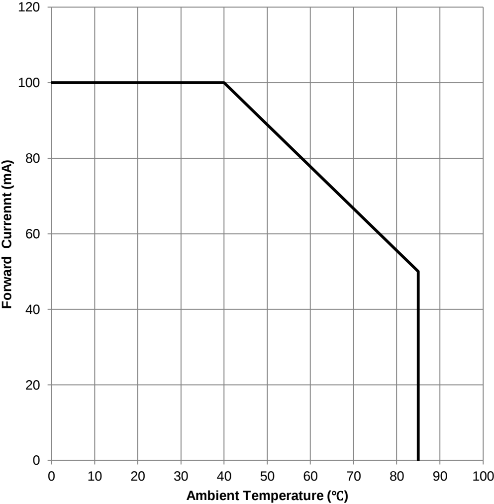
Derating Curve:
