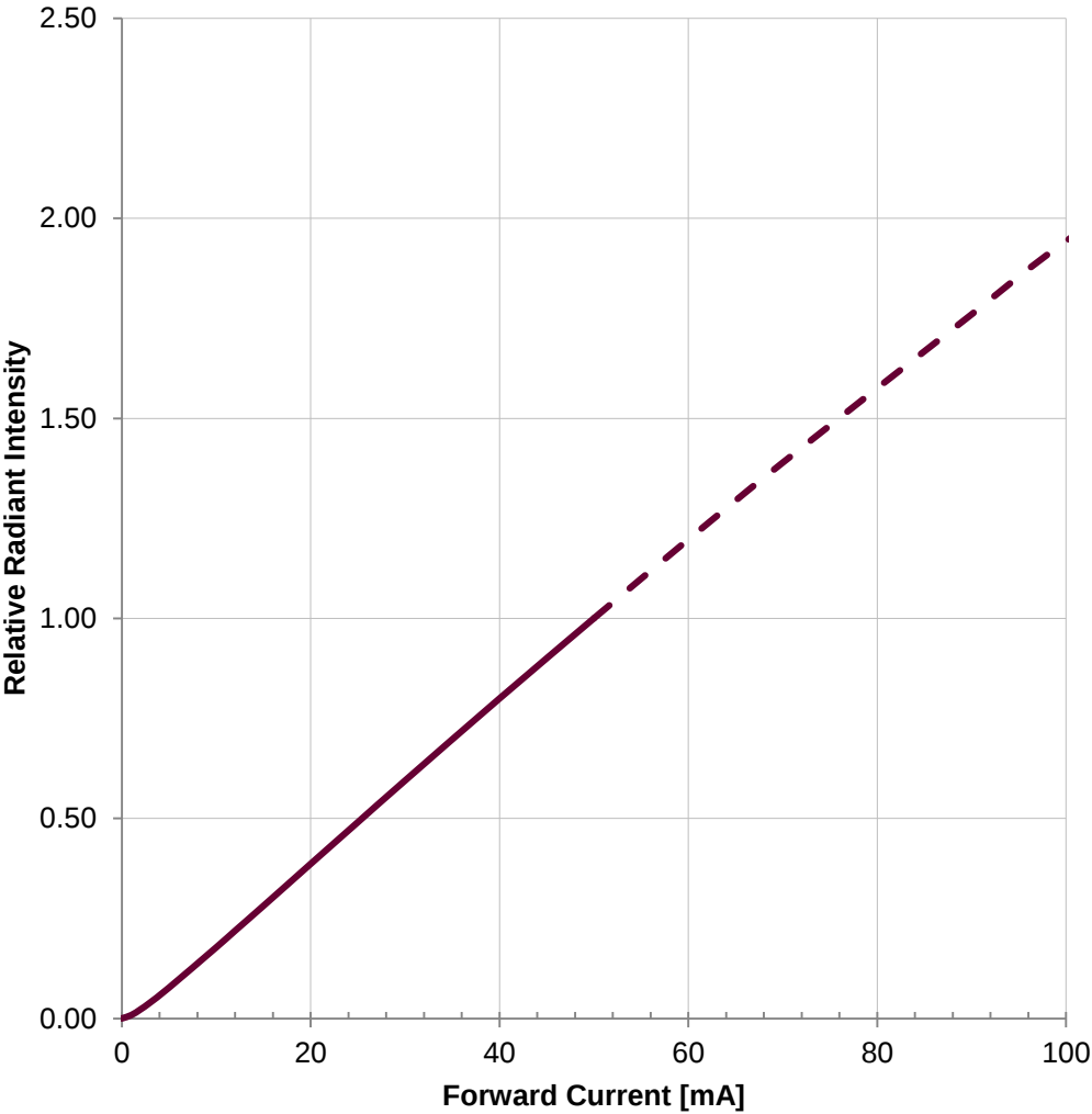
Radiant Intensity vs. Forward Current:
