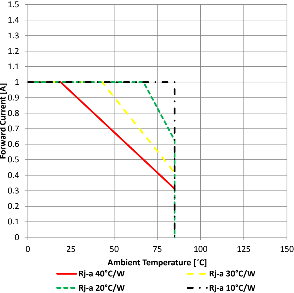
Derating Curve:
