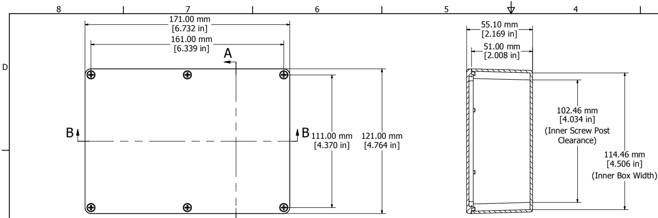
SECTION A-A End View of Assembly
