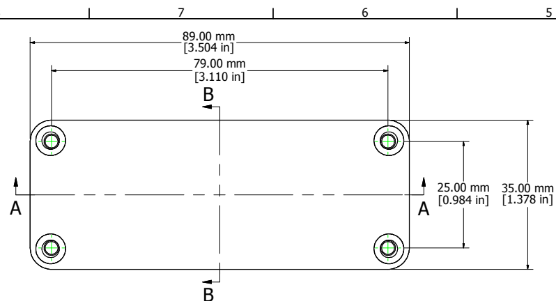
Top View of Assembly
