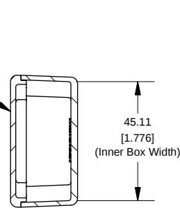
SECTION A-A End View of Assembly
