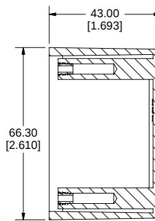
SECTION B-B SCALE 1 : 1
