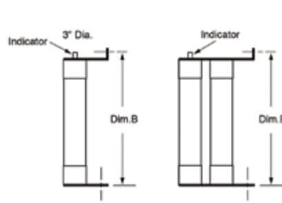
Inverted-Bolt "IB"
