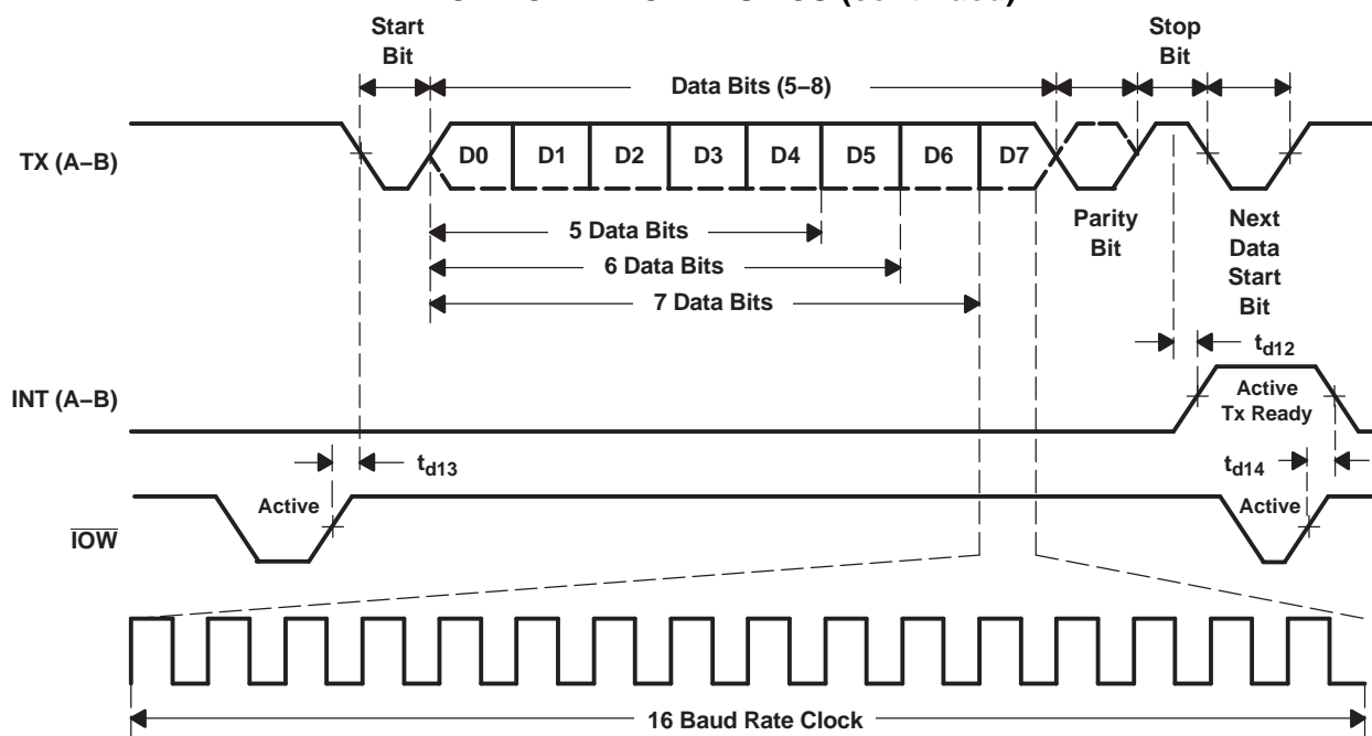
Figure 18. Transmit Timing
