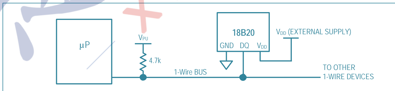
Figure 5. Powering the 18B20 with an External Supply
