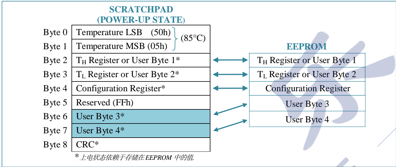
Figure 7. 18B20 Memory Map
