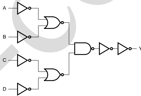
Figure 3. Logic diagram for one gate
