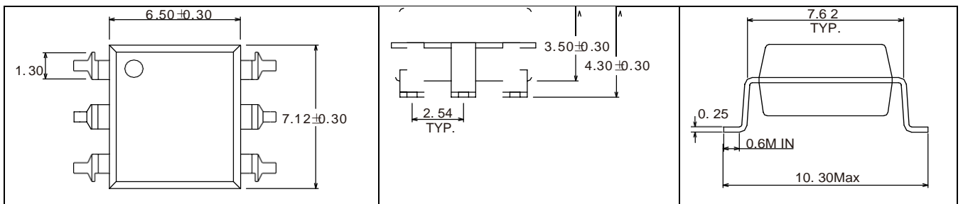
6-pin SOP
