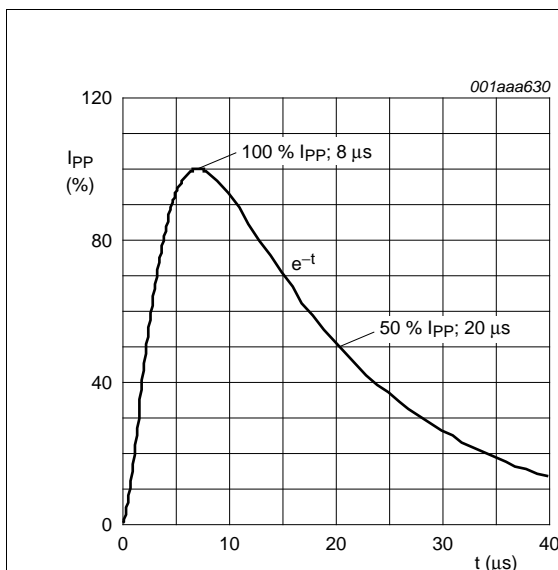
Fig 1. 8/20 μs pulse waveform according to IEC 61000-4-5
