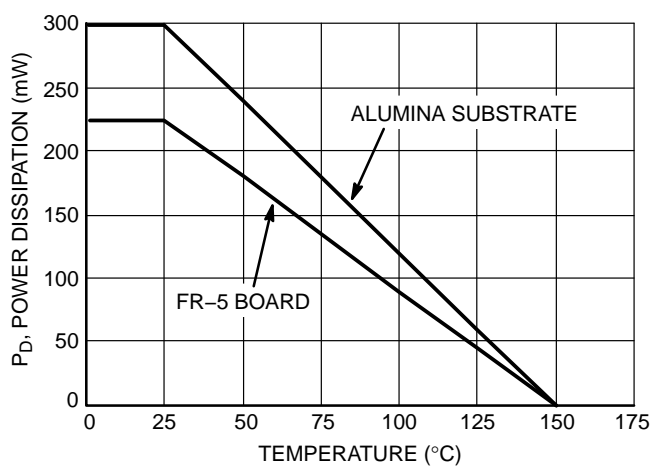
Figure 2. Steady State Power Derating Curve
