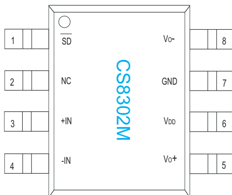
MSOP_8L (Top View)
