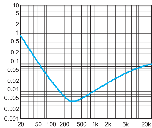
THD+N vs. Frequency SE mode, 6V, 320hm, P_o=70\text{mW}
