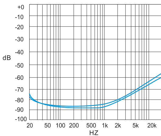
PSRR vs. Freq SE mode, 6V, 320hm, 200mVpp Input terminated
