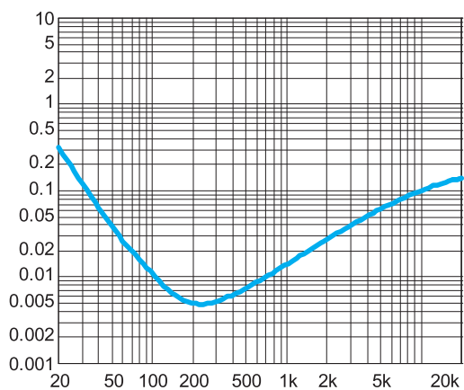
THD+N vs. Frequency SE mode, 3V, 320hm, P_o=20\text{mW}
