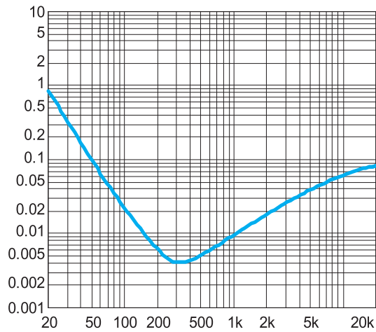
Figure 11. THD+N vs. Frequency SE mode, 6V, 320hm, P_o=70mW
