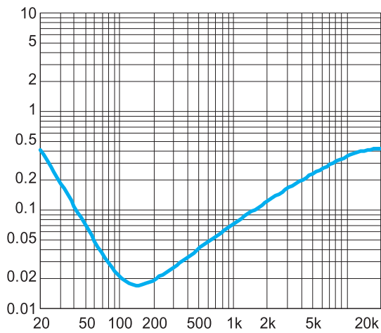
Figure 13. THD+N vs. Frequency BTL mode, 6V, 40hm, P_o=1W
