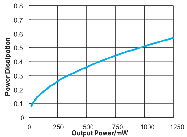
Figure 44. Power Dissipation vs. Output Power BTL mode, 5V, f=1\text{ kHz} , R_L=8\text{ Ohm} , \text{THD+N} \leq 1\%
