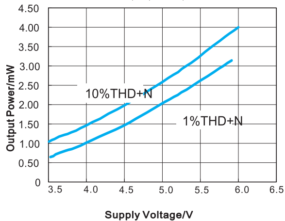
Figure 43. Output Power vs. Power Supply BTL mode, f=1\text{ kHz} , R_L=8\text{ Ohm}
