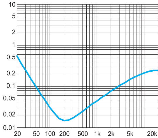
Figure 9. THD+N vs. Frequency BTL mode, 6V, 80hm, P_o=800mW
