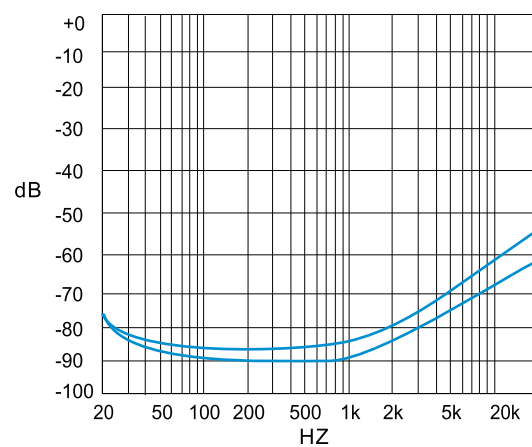
Figure 20. PSRR vs. Freq SE mode, 3V, 320Ohm, 200mVpp Input terminated
