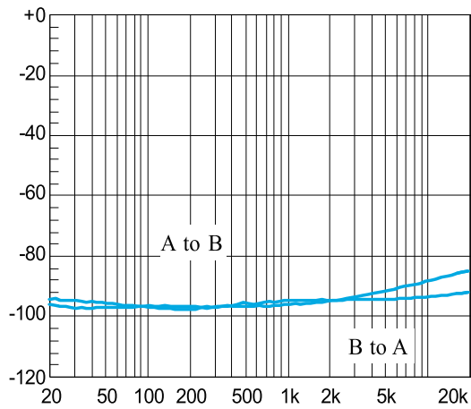
Figure 39. Crosstalk BTL mode, 5V, 8Ohm, Po=1W
