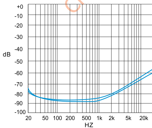
Figure 19. PSRR vs. Freq SE mode, 5V, 320Ohm, 200mVpp Input terminated
