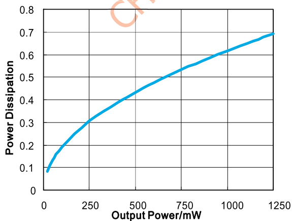
Figure 31. Power Dissipation vs. Output Power BTL mode, 5V, f=1\text{ kHz} , R_L=8\text{ Ohm} , THD+N\leq 1\%
