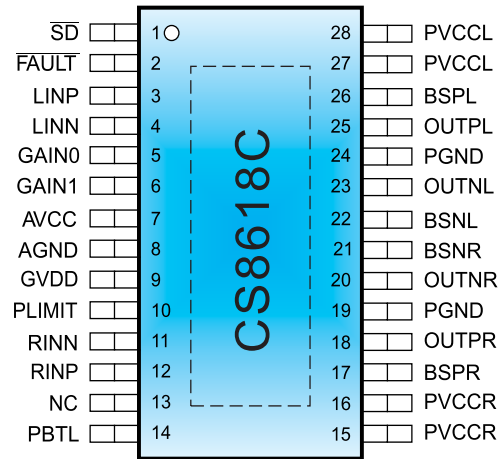
(TSSOP28-PP)PACKAGE (TOPVIEW)
