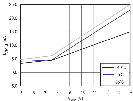
Figure 2. Sleep Current
