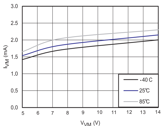
Figure 1. Operating Current
