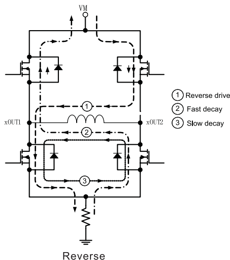
Drive and Decay Modes
