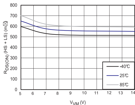
Figure 4. R DS(on) (HS + LS)
