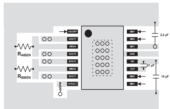
Recommended Layout Example
