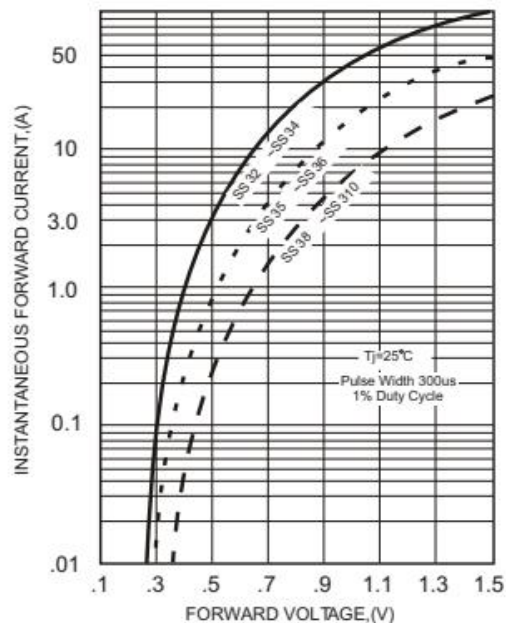
FIG.2-TYPICAL FORWARD CHARACTERISTICS
