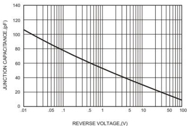
FIG.5-TYPICAL JUNCTION CAPACITANCE
