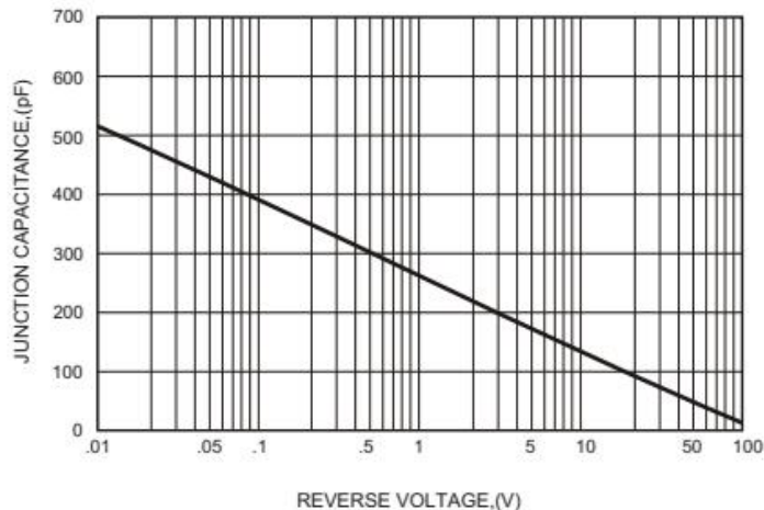
FIG.4-TYPICAL JUNCTION CAPACITANCE
