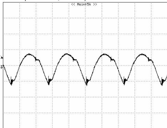
Figure 12: Output voltage ripple at nominal input voltage ( v_{in}=48v ) and rated load current ( I_o=4.2A ) (50 mV/div, 1 us/div). Load capacitance: 1 \mu F ceramic capacitor and 10 \mu F tantalum capacitor. Bandwidth: 20 MHz. Scope measurements should be made using a BNC cable (length shorter than 20 inches). Position the load between 51 mm to 76 mm (2 inches to 3 inches) from the module
