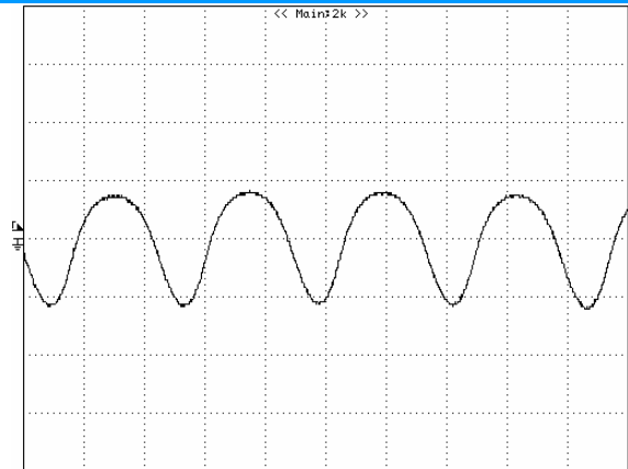
Figure 9: Input Terminal Ripple Current, i_c , at full rated output current and nominal input voltage ( V_{in}=48v ) with 12 \mu H source impedance and 33 \mu F electrolytic capacitor (200 mA/div, 1 us/div)
