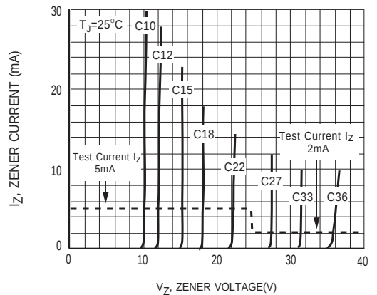
Figure3 Zener Breakdown Characteristics
