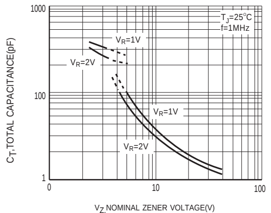
Figure5 Total Capacitance vs Nominal Zener Voltage
