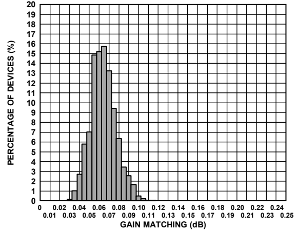
Figure 8. Channel-to-Channel Gain Matching (Gain = 16 dB)
