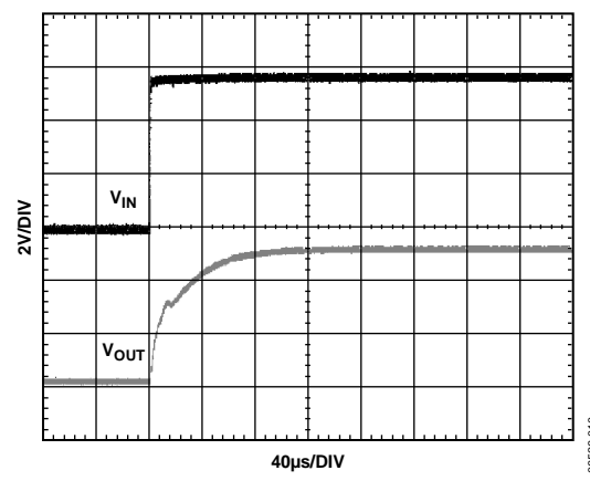
Figure 7. ADR5045 Start-Up Characteristics
