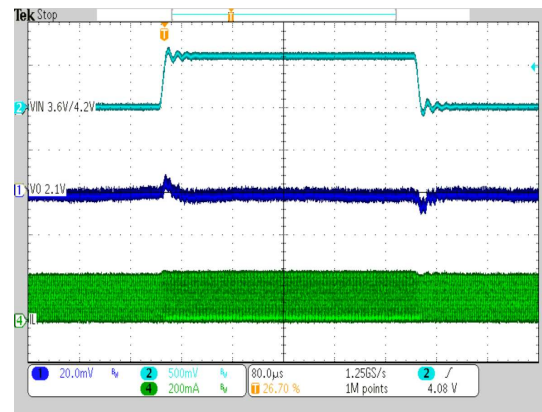
V_{IN} = 3.6\text{ V} / 4.2\text{ V} V_{OUT} = 2.1\text{ V} L = 2.2\text{ }\mu\text{H} C_{OUT} = 10\text{ }\mu\text{F} CTRL = \text{GND}
