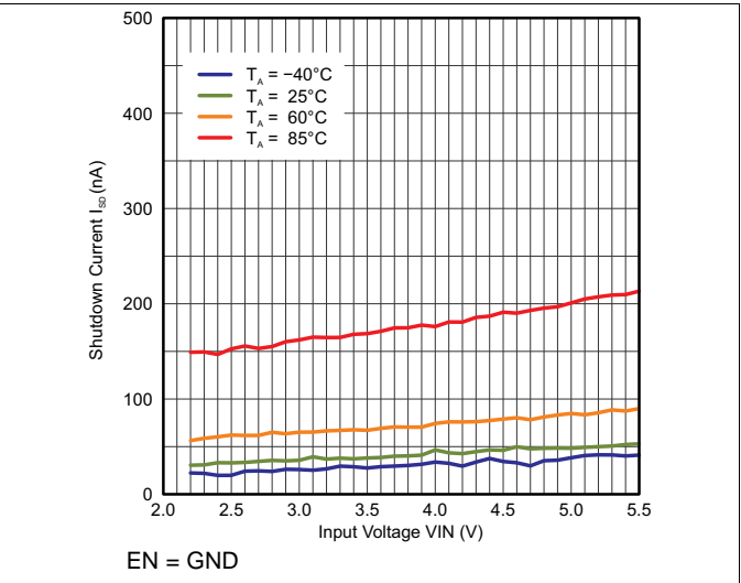
Figure 2. Shutdown Current I_{SD}
