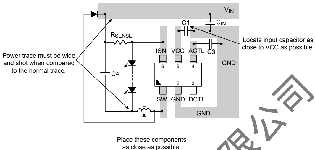
Figure 5. PCB Layout Guide
