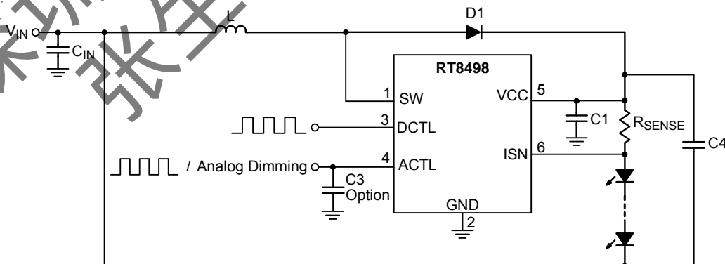
Figure 3. Buck-Boost Configuration
