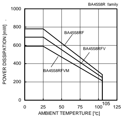
Fig. 23 Derating Curve
