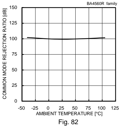
Fig. 82 Common Mode Rejection Ratio - Ambient Temperature (VCC/VEE=+15[V]/-15[V], Vicm=-12[V] to +12[V])
