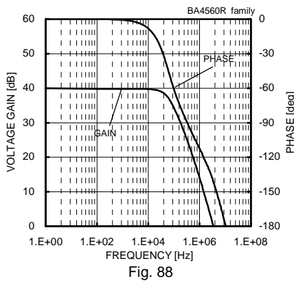
Fig. 88 Voltage Gain - Frequency (VCC/VEE=+15[V]/-15[V], Av=40[dB], RL=2[kΩ], Ta=25[°C])
