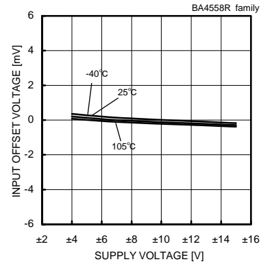
Fig. 31 Input Offset Voltage - Supply Voltage (Vicm=0[V], Vout=0[V])
