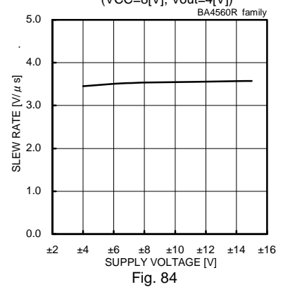
Fig. 84 Slew Rate - Supply Voltage (CL=100[pF], RL=2[kΩ], Ta=25[°C])
