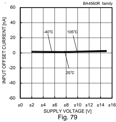
Fig. 79 Input Offset Current - Supply Voltage (Vicm=0[V], Vout=0[V])
