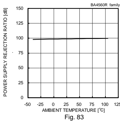
Fig. 83 Power Supply Rejection Ratio - Ambient Temperature (VCC/VEE=+4[V]/-4[V] to +15[V]/-15[V])
