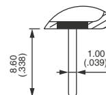
Straight PC
