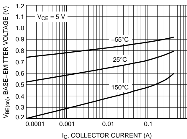
Figure 19. Base Emitter Voltage vs. Collector Current
