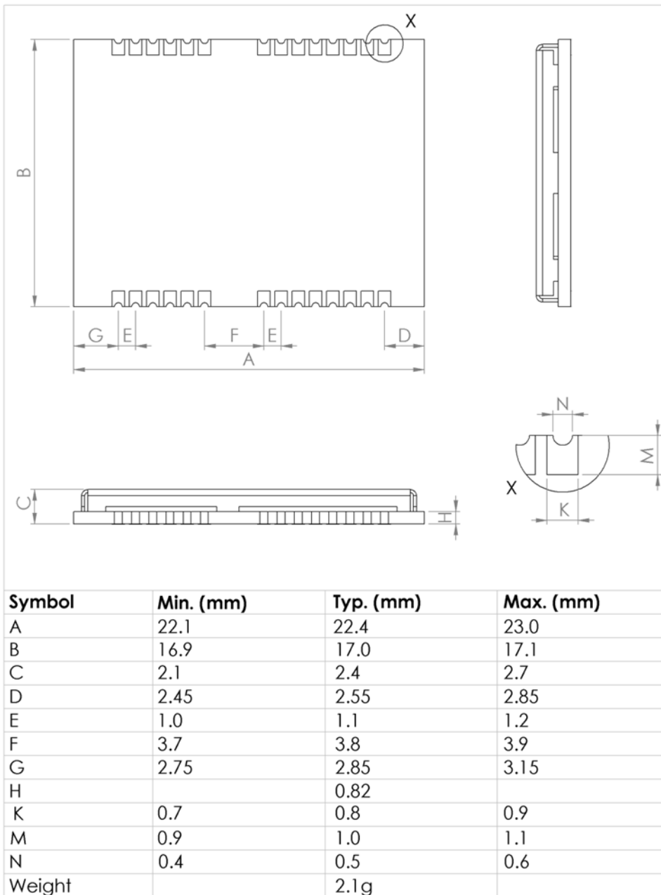
Figure 7: LEA dimensions
