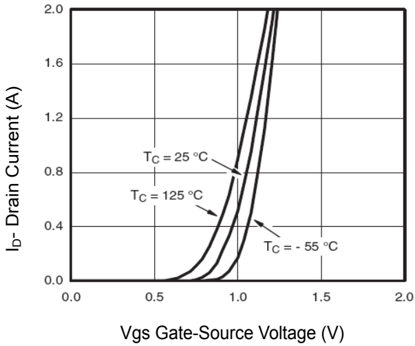
Figure 7 Transfer Characteristics
