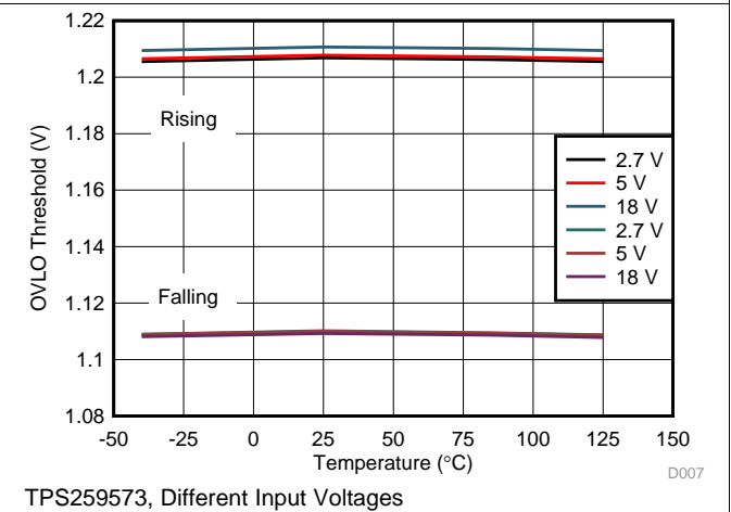
Figure 8. OVLO Threshold vs Temperature
