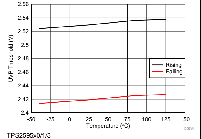
Figure 6. UVP Threshold vs Temperature
