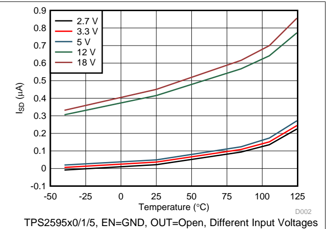
Figure 4. Shutdown Current vs Temperature
