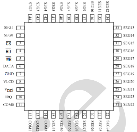
QFP44
