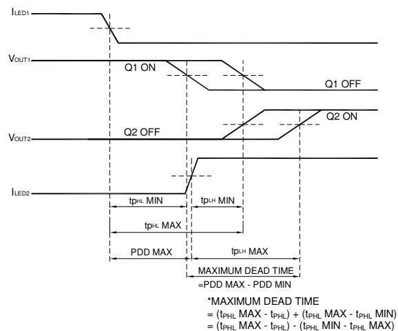
Figure 27 : Waveforms for dead time
