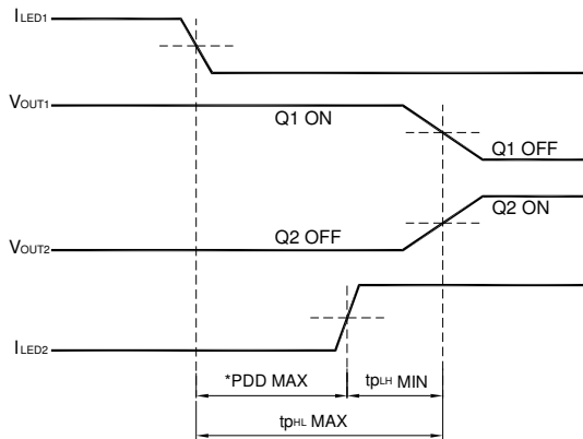
Figure 26 : Minimum LED skew for zero dead time
