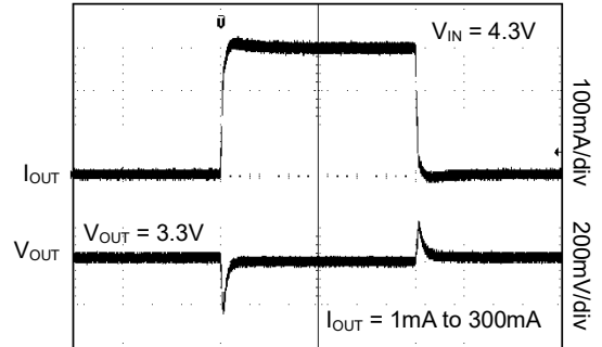
Time (100μs/div)
