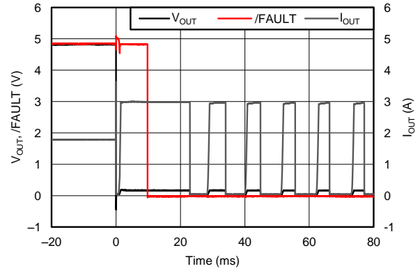
Figure 26. 2.5 Ω to Output Short Transient Response
