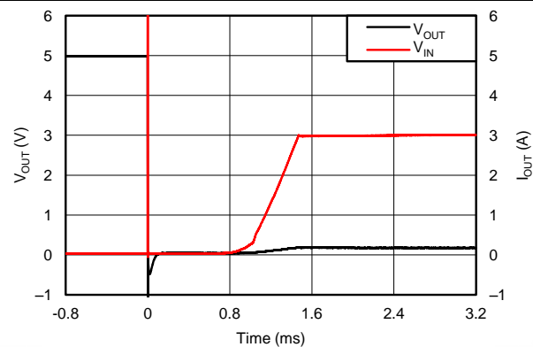
Figure 28. No Load to Output Short Transient Response
