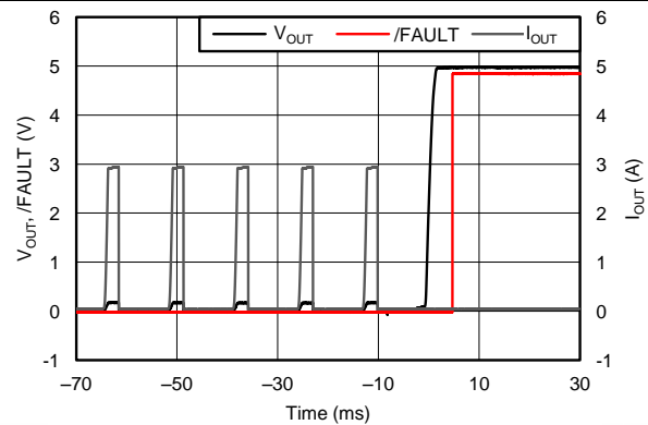
Figure 27. Output Short to 2.5-Ω Load Recovery Response
