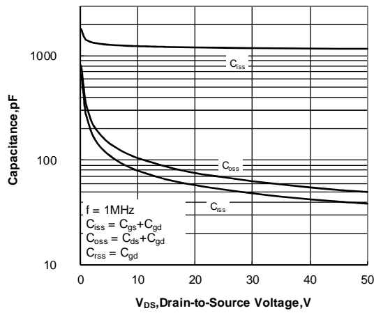
Figure 12. Capacitance Characteristics
