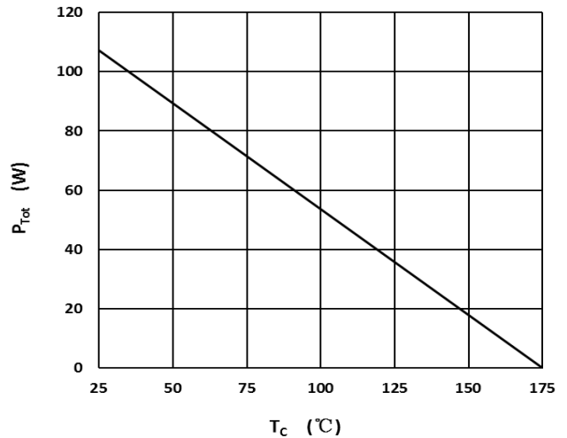
Fig 4: Power Derating
