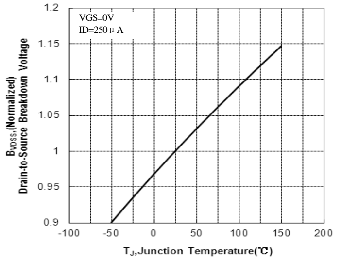
Figure 11 Typical Breakdown Voltage vs Junction Temperature
