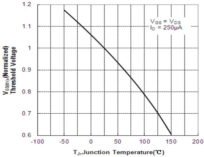
Figure 10 Typical Theshold Voltage vs Junction Temperature
