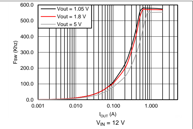
Figure 8. TPS562201 Switching Frequency vs Output Current
