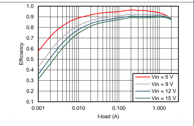
Figure 10. TPS562201 V_{OUT} = 1.5\text{ V} Efficiency, L = 2.2\ \mu\text{H}
