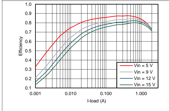
Figure 9. TPS562201 V_{OUT} = 1.05\text{ V} Efficiency, L = 2.2\ \mu\text{H}
