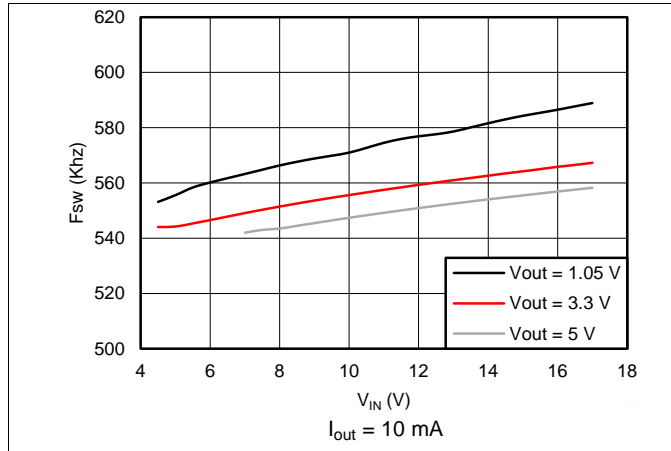
Figure 7. TPS562208 Switching Frequency vs Input Voltage
