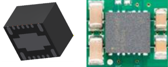
RLF Package and Typical Layout
