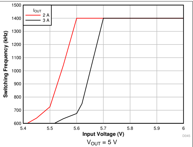
Figure 34. Frequency Foldback
