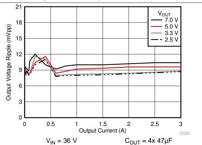
Figure 22. Voltage Ripple versus Output Current
