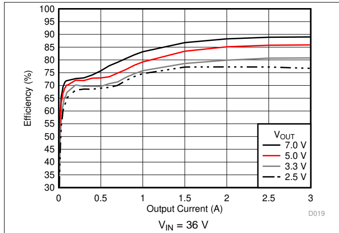
Figure 19. Efficiency versus Output Current
