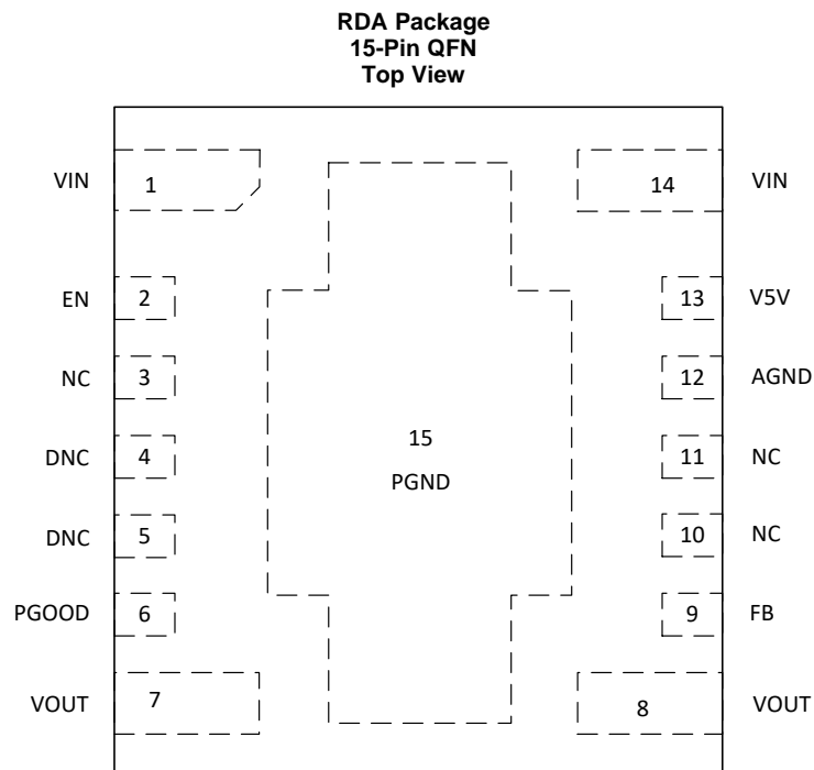
Pin Functions
