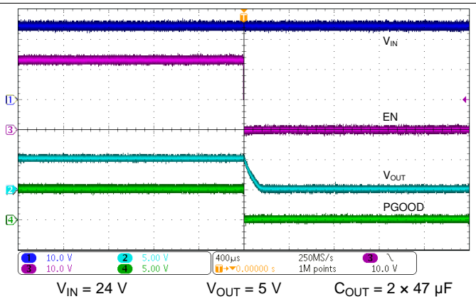
Figure 42. Enable Turn-OFF
