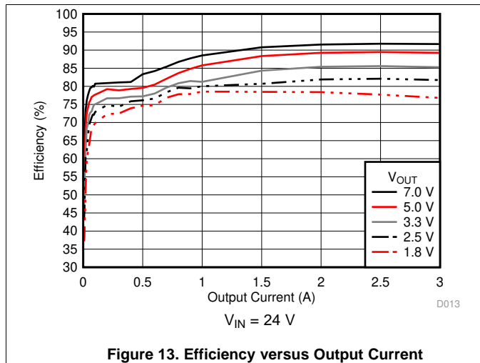
Figure 13. Efficiency versus Output Current
