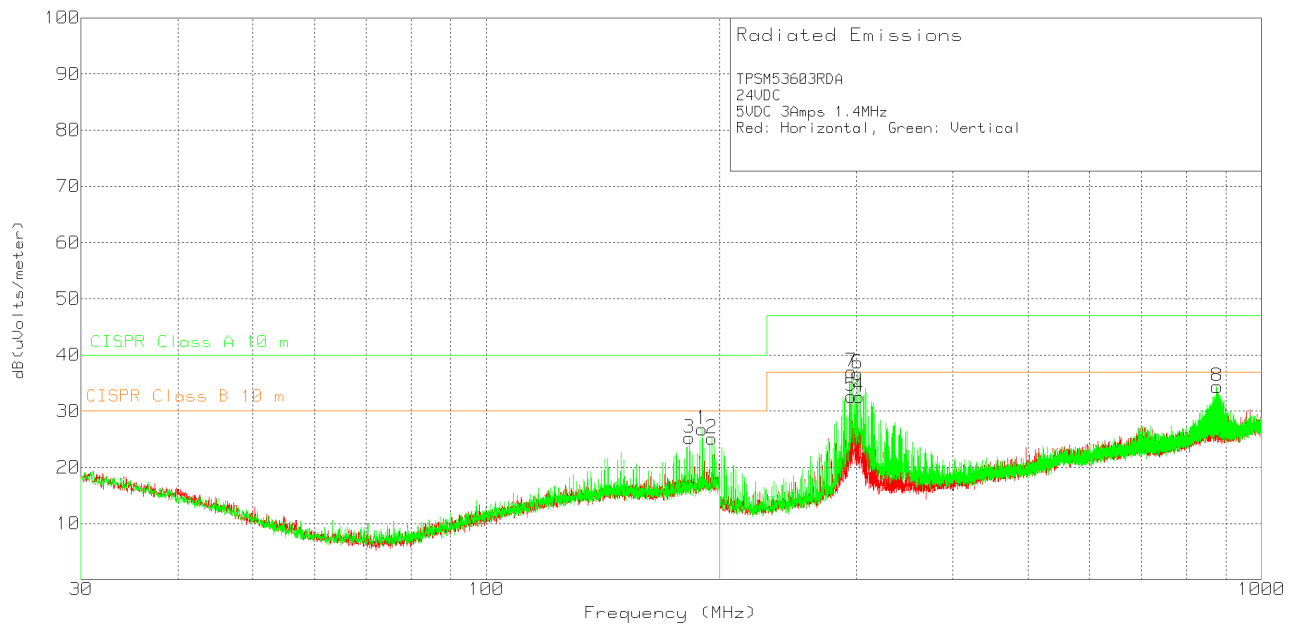
Figure 48. Radiated Emissions 24-V Input, 5-V Output, 3-A Load
