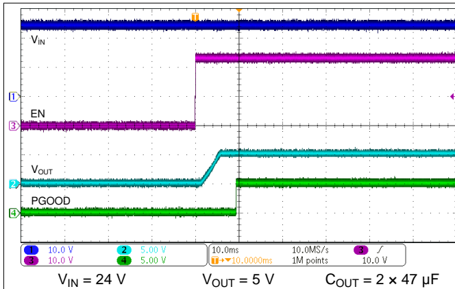
Figure 41. Enable Turn-ON
