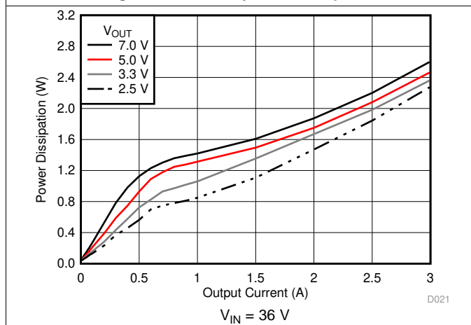
Figure 21. Power Dissipation versus Output Current
