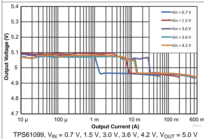
Figure 9. Load Regulation
