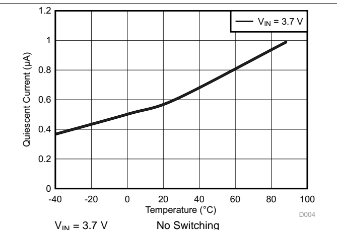
Figure 10. Quiescent Current into V_{OUT} vs Temperature
