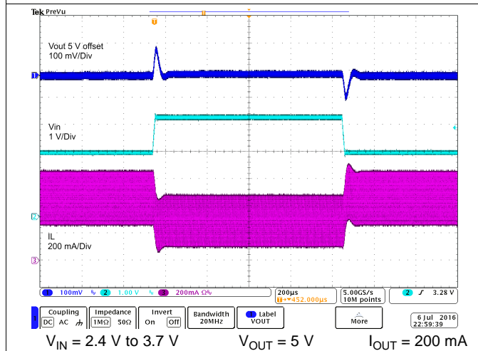
Figure 25. Line Transient
