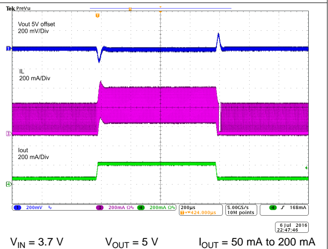
Figure 26. Load Transient
